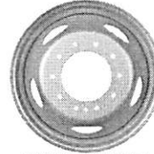
19.5" Argent Painted Steel (19.5"x6"; hub cover/center ornament not included; Std. on XL and XLT F-450 and F- 550) – 64Z
